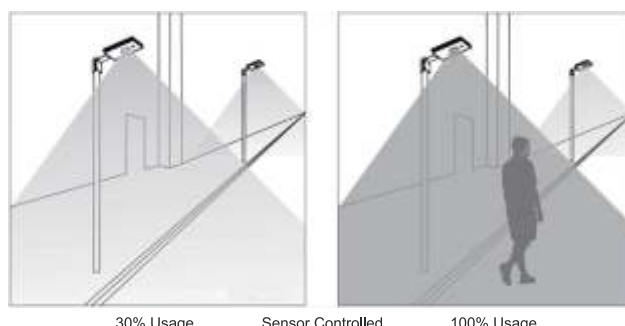
30% Usage Sensor Controlled 100% Usage When nobody around the light, it works at 30% power automatically. When people pass by, the motion sensor detects it and the light will be at 100% power.
