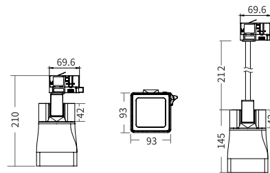
4-pin track adaptor
