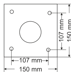
Mounting plate
